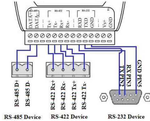
Figure 4: Serial port wire connection
