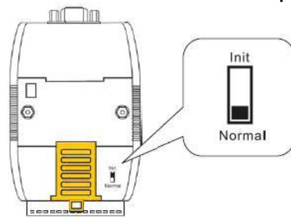
Figure 2: Operation mode Position of Dip-Switch
