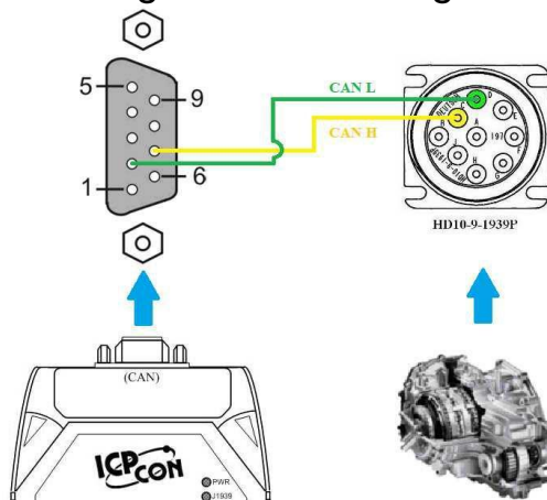
Figure 3: CAN bus Wire Connection
