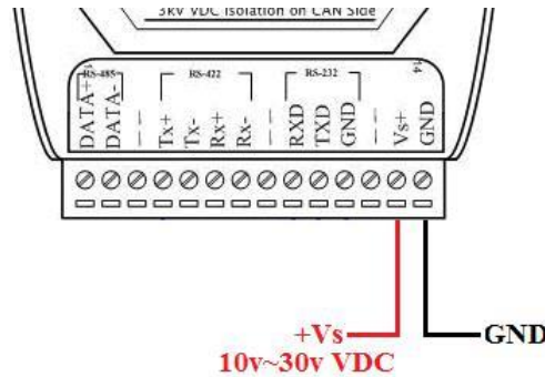
Figure 5: Power Wire Connection
